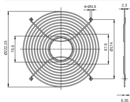
FG-25 For 254mm Fan
